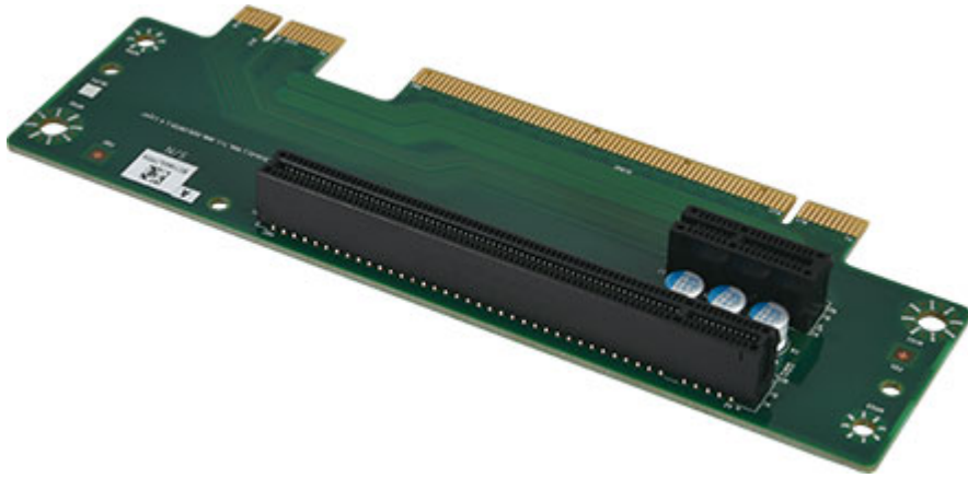
Mitac MX1-10FEP-D Riser (1x PCI-E x1 + 1x PCI-E x16) [MP-116RCN-P10]
